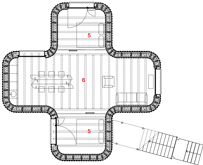
GROUND MEZZANINE FLOOR PLAN
