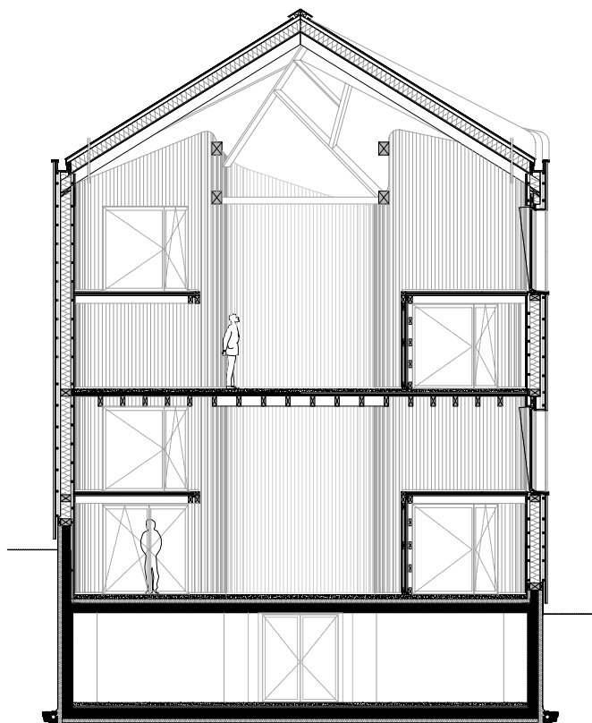
SECTION
